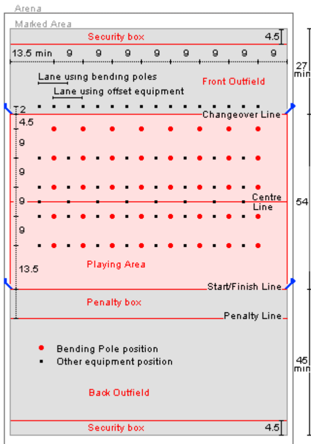
Figure 1 : Arena areas and markings
